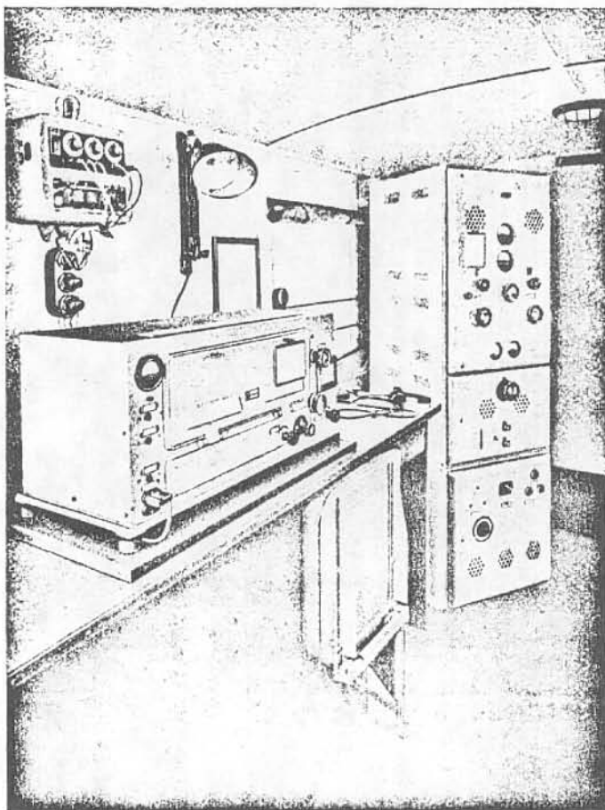
Fahrbare 200-Watt-Langwellen-Station.
